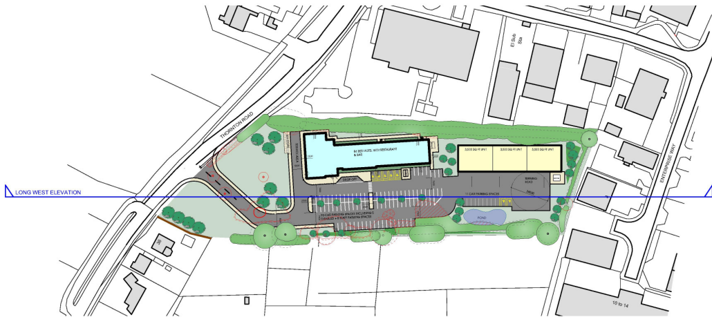
Site Plan Extract (1:1000)
